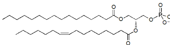
molecule P
