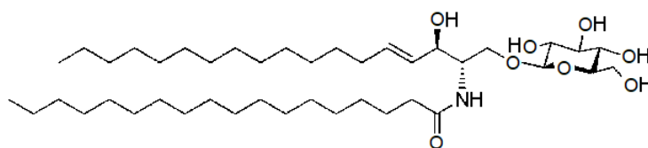
molecule Q
